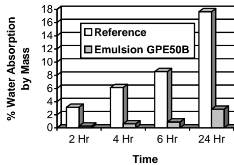
Figure 2. Water absorption of cement render coated with acrylic primer containing Emulsion GPE50B
